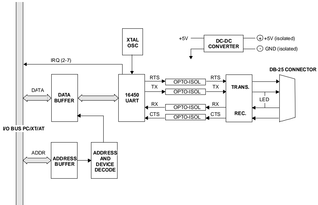
Figure 1: RS422I-P Block Diagram
