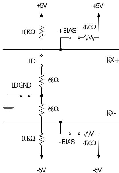
Figure 2: CTS Jumper
